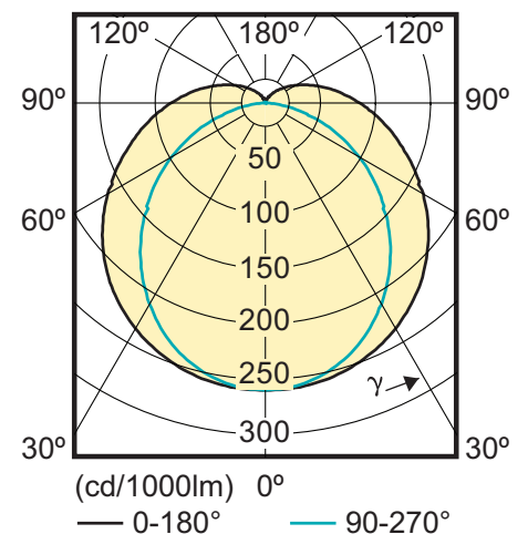
LEDtube 900mm 15W T8C Rot
