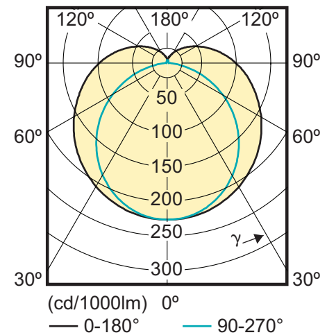
VLE 1500 mm 23 W /865 ROT
