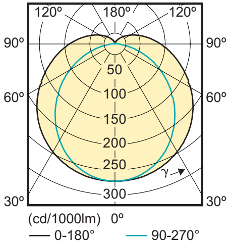
LED tube VLE 600 mm 10 W T8C Rot
