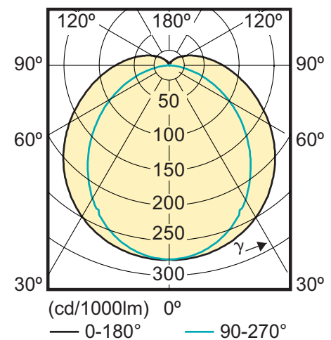
VLE 1500 mm 20 W /865 T8 C
